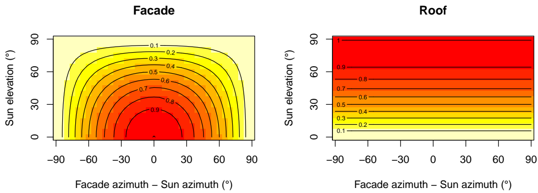
Figure 5: Coefficient of Direct Normal Irradiance, as function of solar position, expressed as the difference between facade and sun azimuths (X-axis) and sun elevation (Y-axis). The left panel refers to a facade, the right panel refers to a roof. Note that a horizontal roof has no azimuth, thus the X-axis is irrelevant for the right panel and only shown for uniformity
