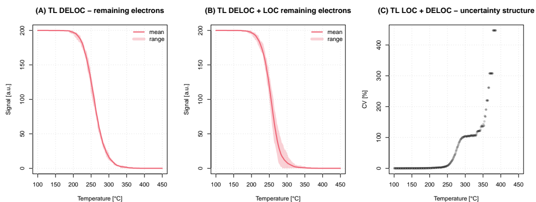
Figure 6: (A) Plot of the remaining electrons for the TL process using the delocalized transition model for which we show the luminescence signal in Figure 5A. (B) Plot of remaining electrons for two models combined in one system. (C) Stochastic uncertainty structure from (B).
