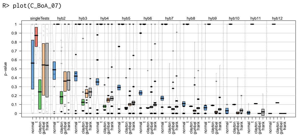
Figure 16: p -values of the C/BoA data for 2007.
