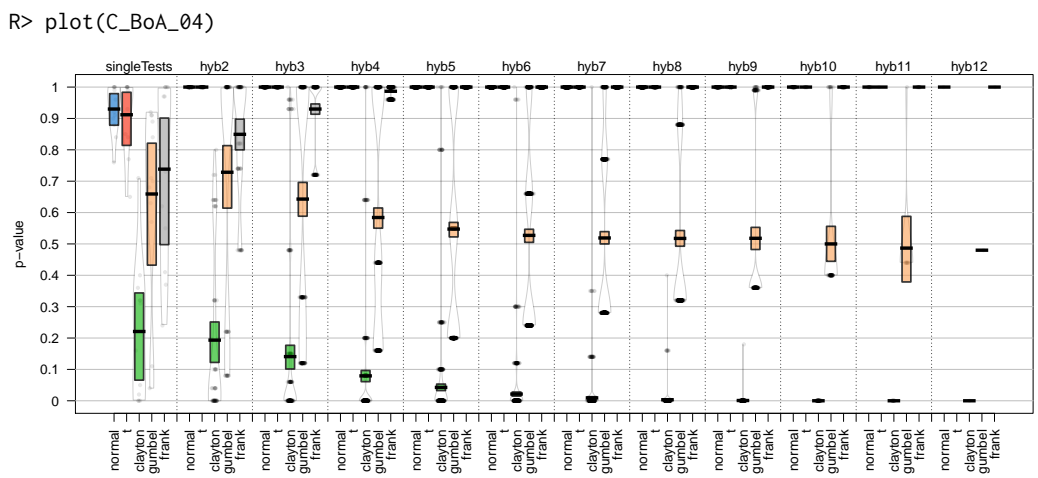
Figure 15: p -values of the C/BoA data for 2004. The column hyb12 of the t -copula is empty, as the p -value of the test gofWhite could not be computed due to instability in the test statistics. For a detailed description of this phenomenon, see Nagler et al. (2019).
