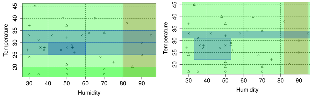
Figure 1: Illustration of postpruning algorithm (HumTemp dataset). Left: CBA model; right: QCBA model.
