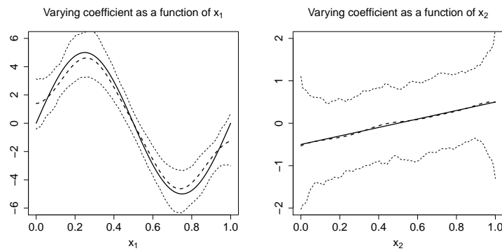
(b) Bernoulli
