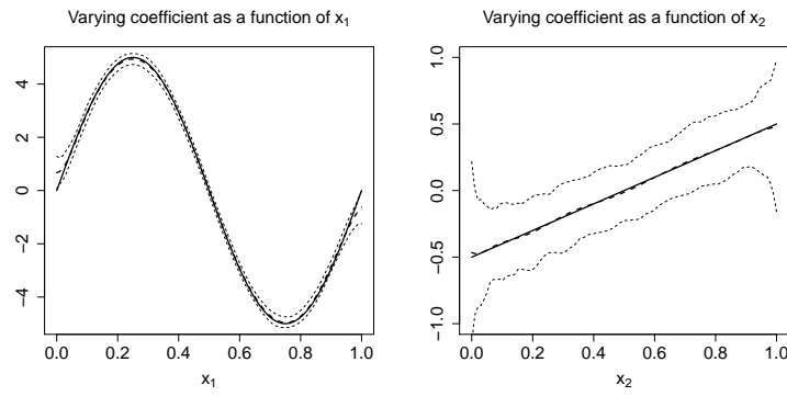
(a) Gaussian
